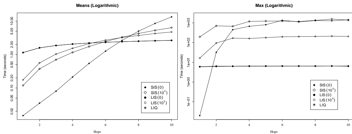
Figure 3: Latency experienced by packets that cross 10 links with policies LIS, SIS, and LIQ under distribution of skews with different standard deviations.
