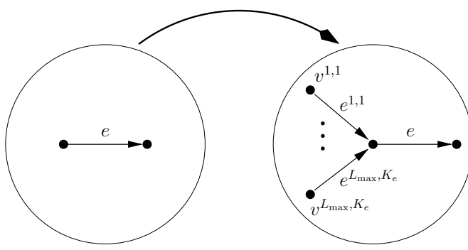
Figure 2: Basic process to transform \mathcal{G} into \mathcal{G}' .
