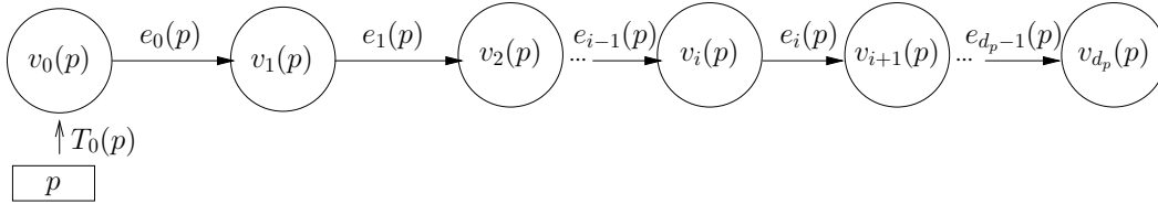
Figure 1: Path \Pi(p) assigned to a packet p in the network.
